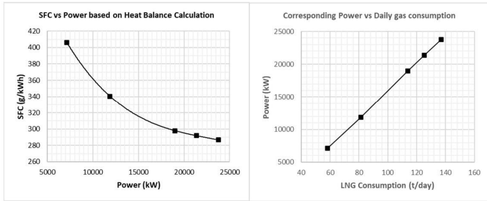
Figure 1 Example of SFC vs Power from heat balance and Corresponding Power vs Daily Gas Consumption curves for a typical steam ship
