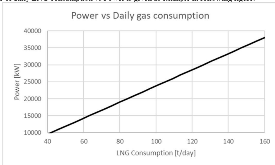
Figure 2 Example of daily LNG consumption vs Power for a typical DFDE ship
