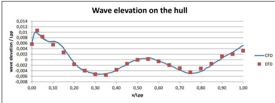
Figure 8.2.4-1 Free surface wave diagram
