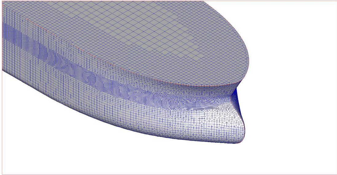
Figure 6.2-3 Meshing at bow
