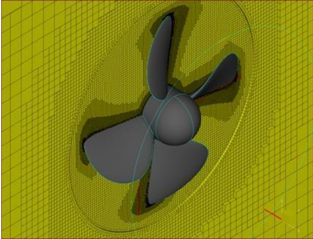
Figure 6.2-5 Meshing in way of appendage
