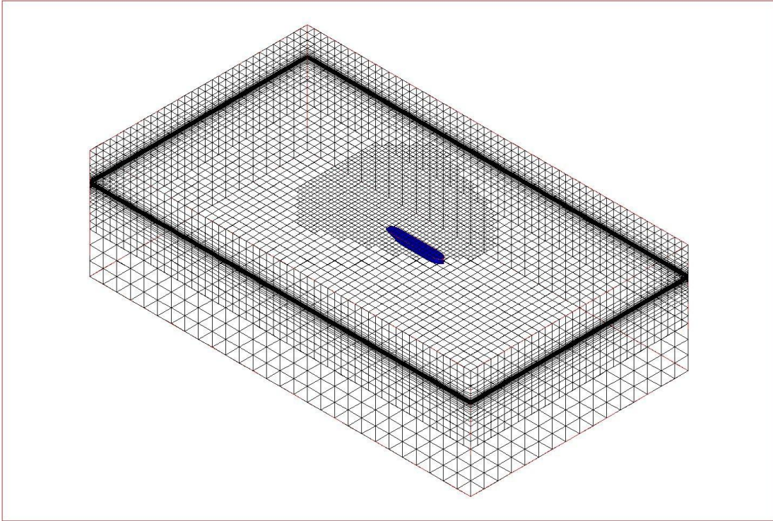
Figure 6.2-1 Division of calculation domain
