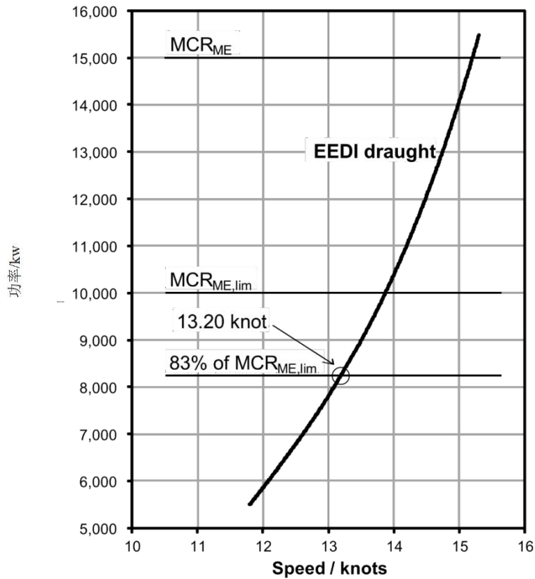
Figure 2.1: Power curve
