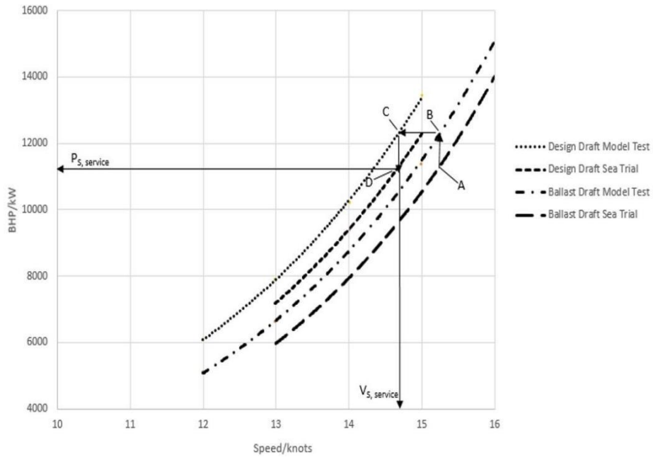
Figure 2.2: Power curve
