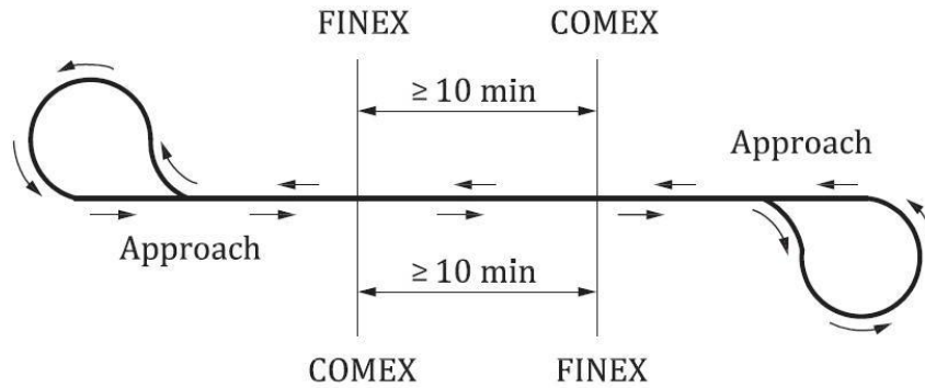
Figure 1: Sea trials with double runs
