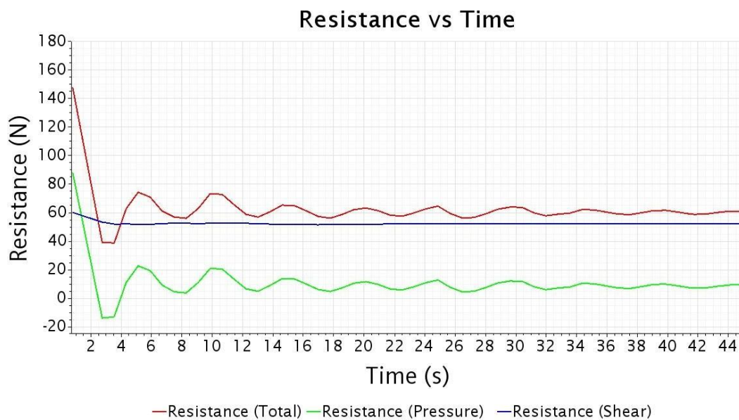
Figure 8.2.3 Convergence Plot of Main Efforts (example of resistance)
