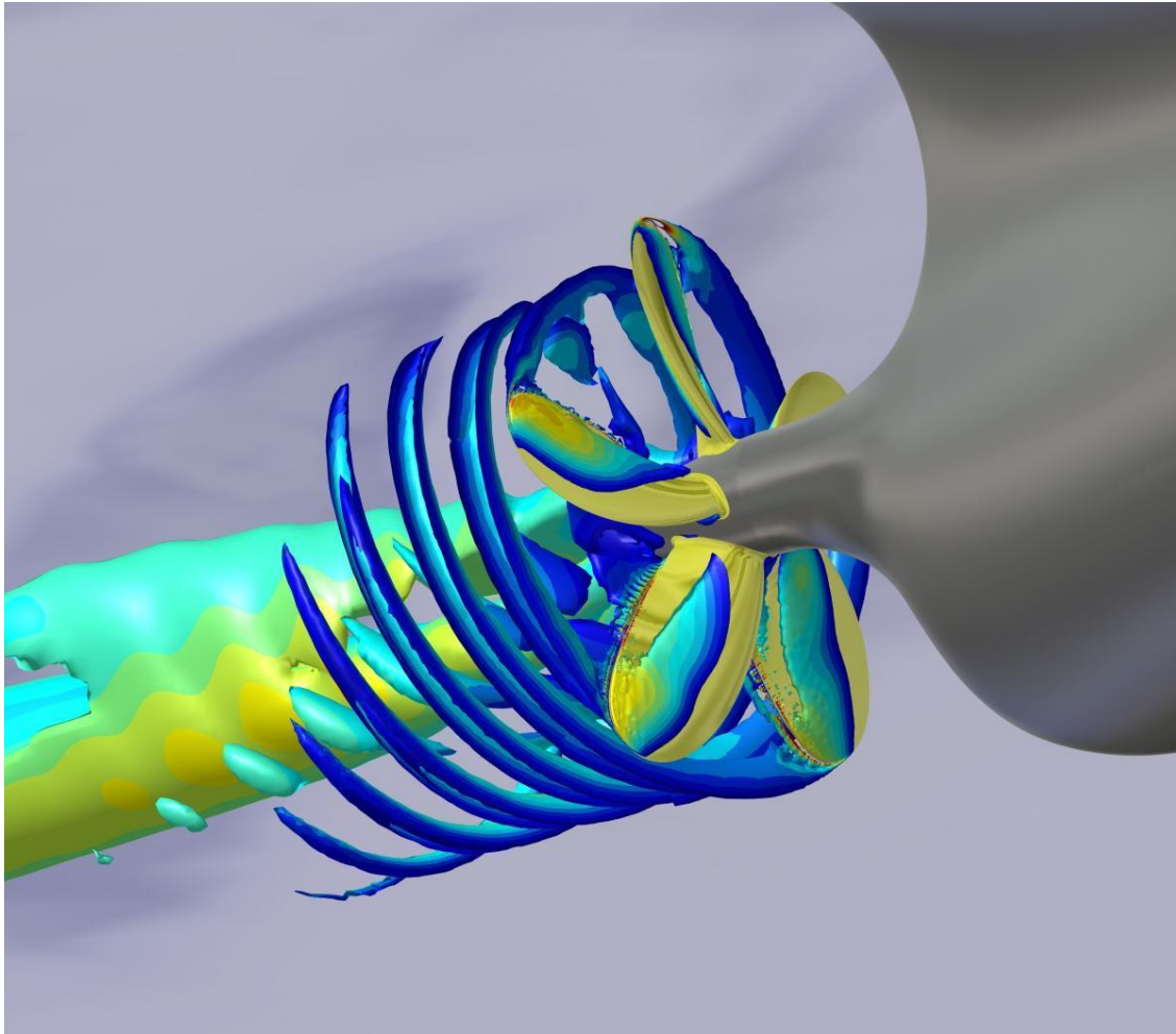
Figure 8.2.4-4 Distribution of flow field in way of propeller
