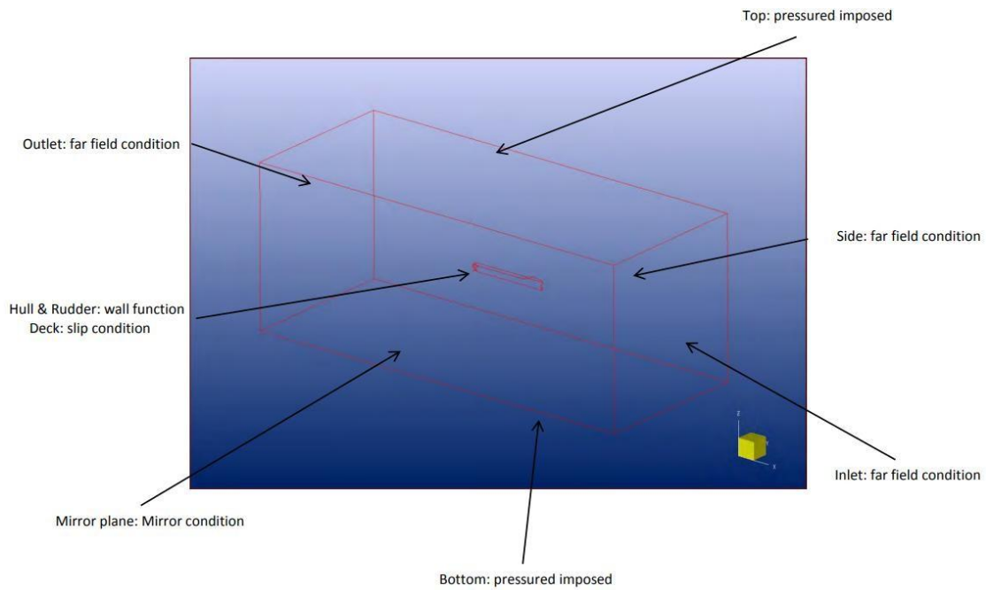
Figure 7.5 Calculation boundary condition set-up
